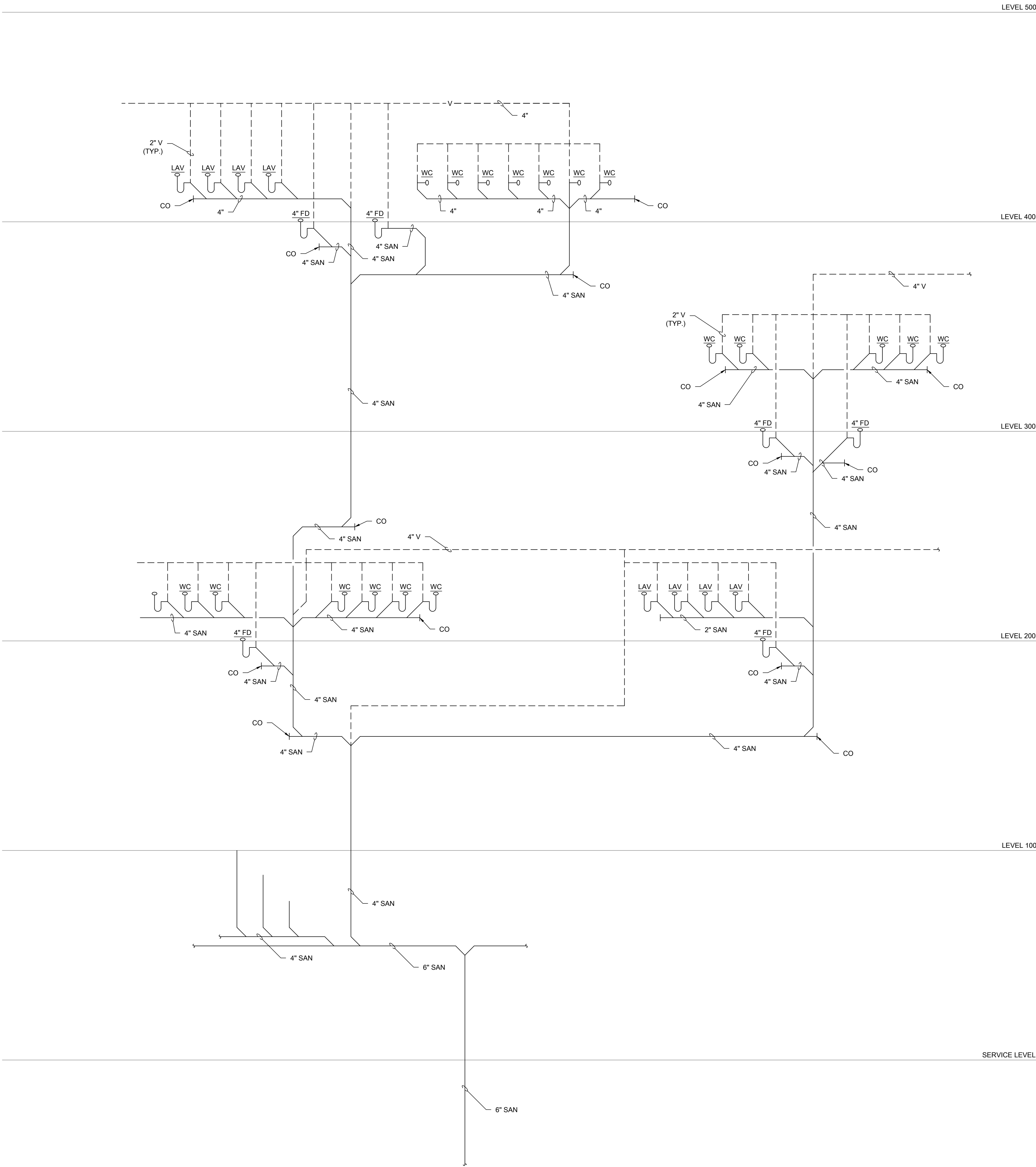
1 PLUMBING DEMOLITION RISER DIAGRAM
